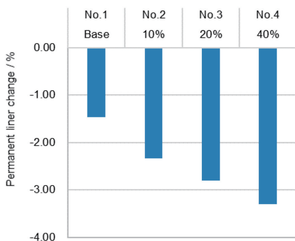
Fig.2 Permanent liner change after firing at 1400℃ for 3hours.
