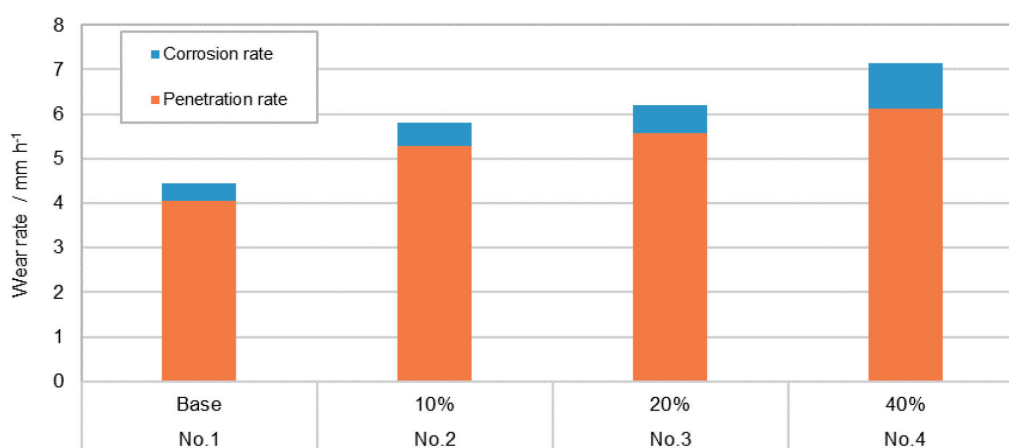
Fig.6 Results of corrosion test.
