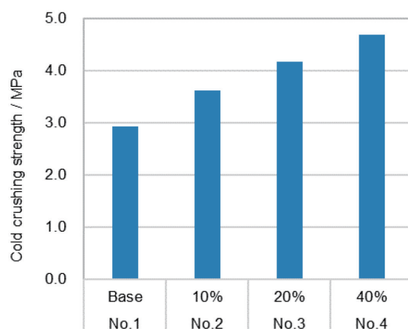
Fig.1 Cold crushing strength after firing at 1400℃ for 3hours.
