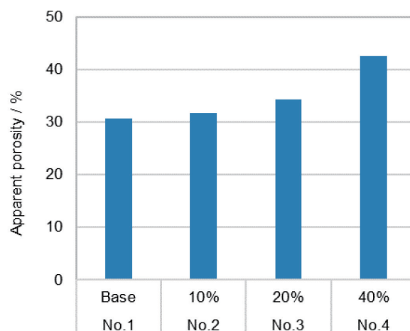
Fig.3 Apparent porosity after firing at 1400℃ for 3hours.
