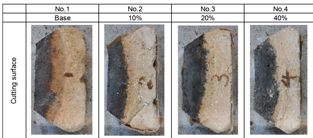
Fig.5 Appearance of cutting surface after corrosion test
