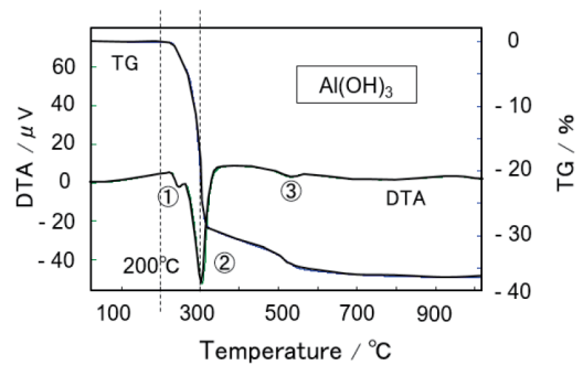
Fig.4 Result of TG-DTA analysis of \text{Al}(\text{OH})_3 .
