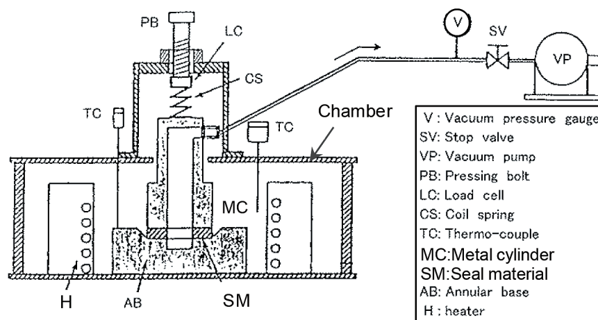
Fig.7 Cross section of the testing apparatus 1) .
