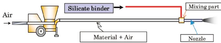
Fig. 1 Schematic of Drying Free gunning system Process.
